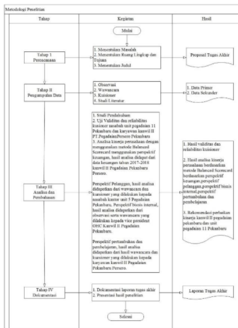
Gambar C.1 Metodologi penelitian
