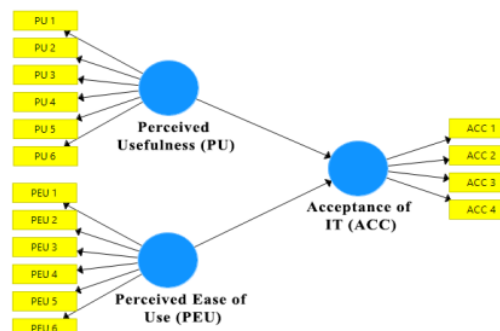
Gambar 4. Path Diagram
