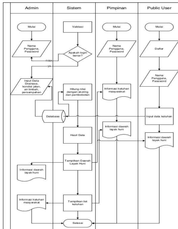
Gambar 1. Flowchart Sistem Usulan
