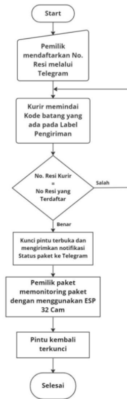
Gambar 5. Flowchart Smart Packages Box
