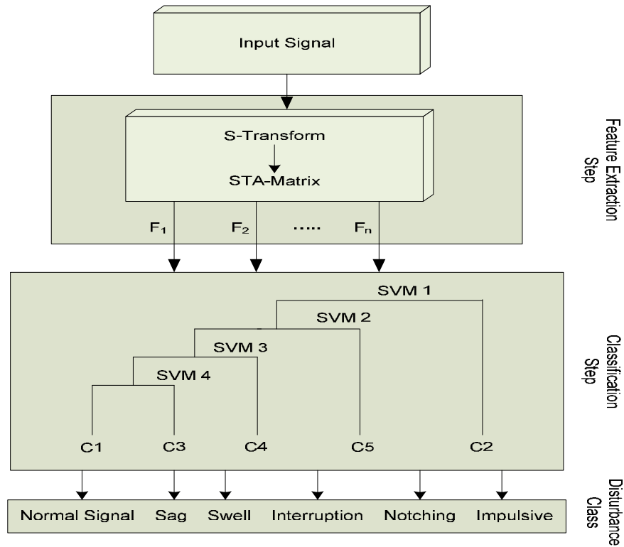
Figure 5. Block Diagram of the Propose System
