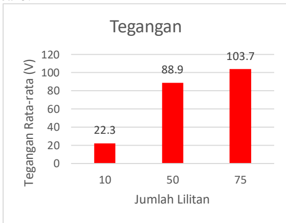
Gambar 3. Tegangan Generator Berbeban
