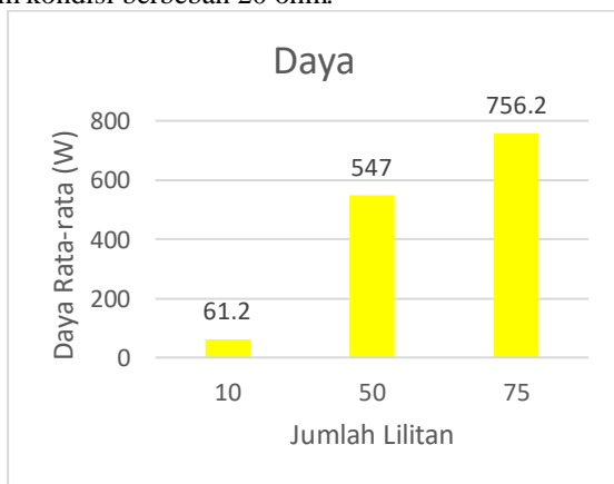
Gambar 4. Daya Generator Berbeban
