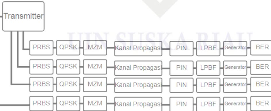
Gambar 5. Blok Diagram Transmitter Modulasi EA
