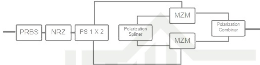
Gambar 6. Blok Diagram Transmitter Modulasi PoISK
