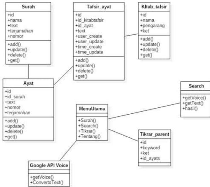
Gambar 5. Class Diagram
