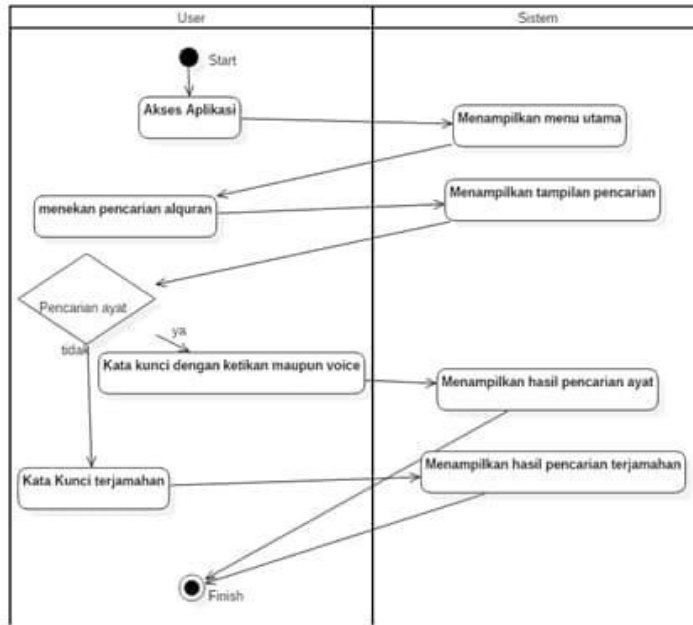
Gambar 4. Activity Diagram
