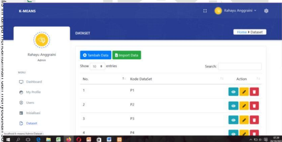
Gambar 3. Halaman Dataset
