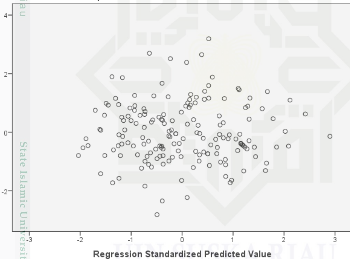
Scatterplot Dependent Variable: IntensiPerilaku
