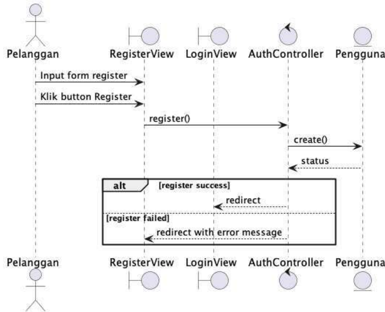
Gambar 4. 11 Sequence Diagram Register Akun Pelanggan
