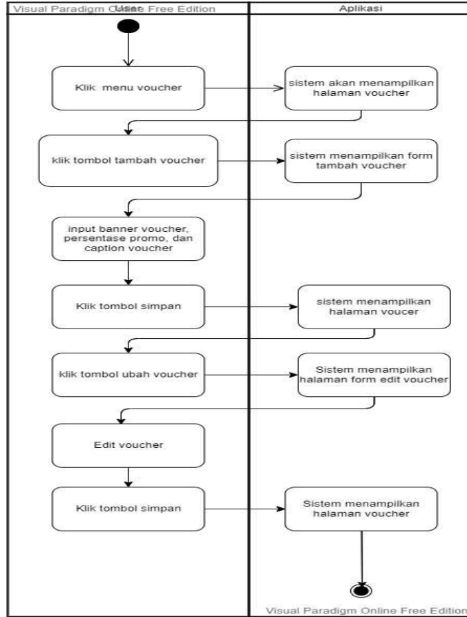
Gambar 4.7 Activity Diagram Mengelola Voucher
