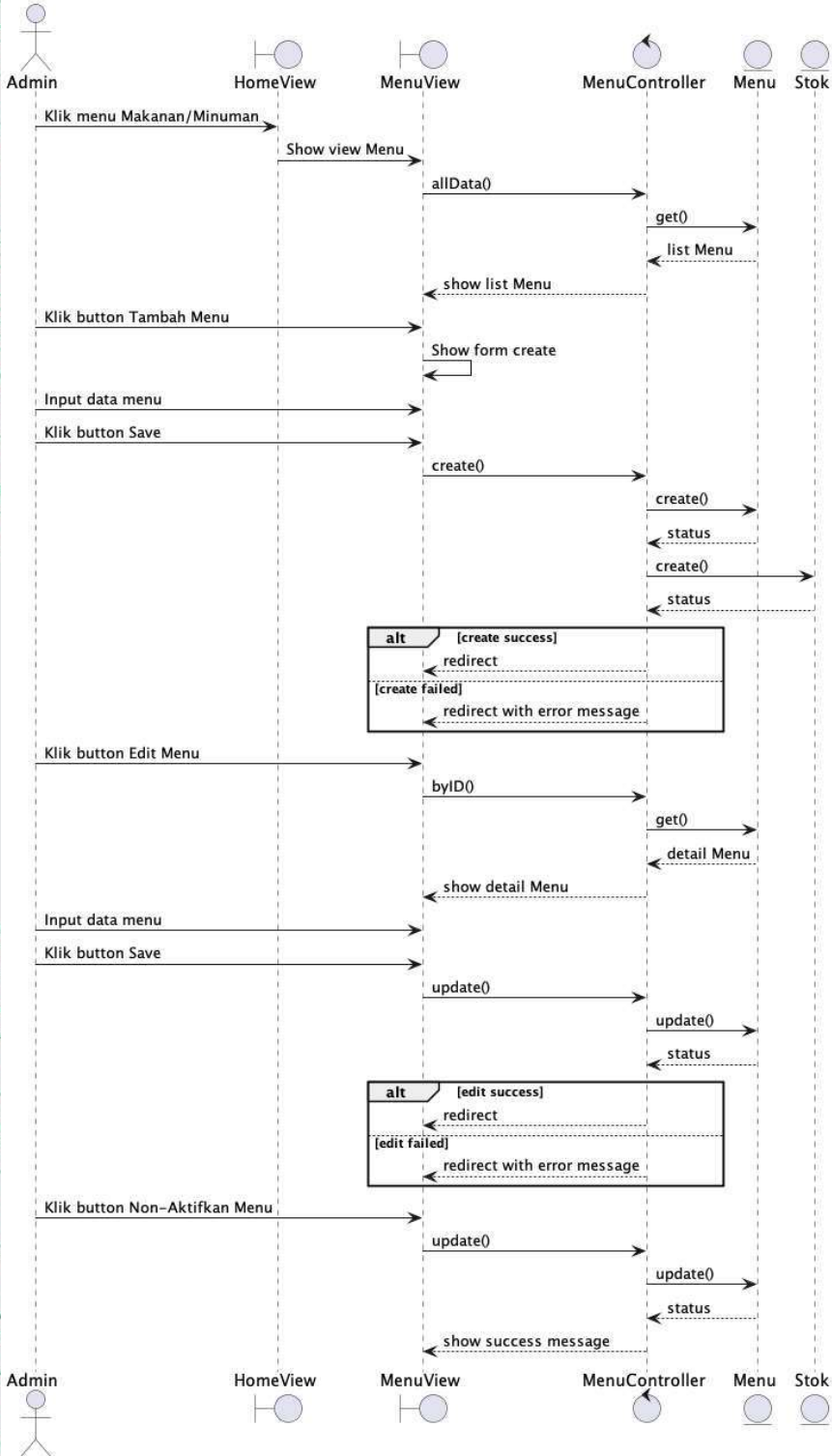
Gambar 4. 13 Sequence Diagram Mengelola Data Menu
