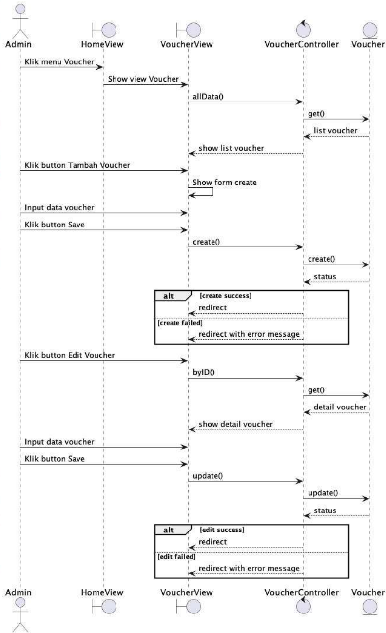
Gambar 4. 16 Sequence Diagram Mengelola Voucher Promo
