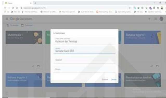
Gambar III.3. Create Class
