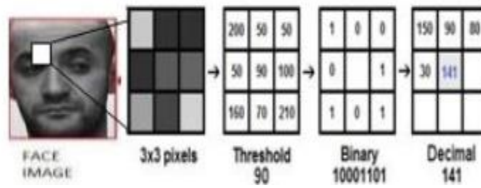
Figure 2. Local Binary Pattern Histogram Method [17].
