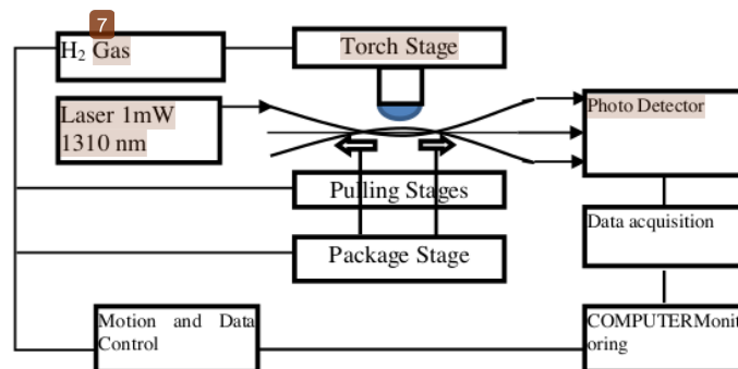
Fig 1. Experimental set up to fabricate fiber coupler
