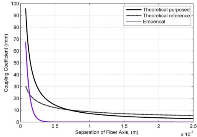
Fig 2. Coupling coefficient versus separation between fiber axis
