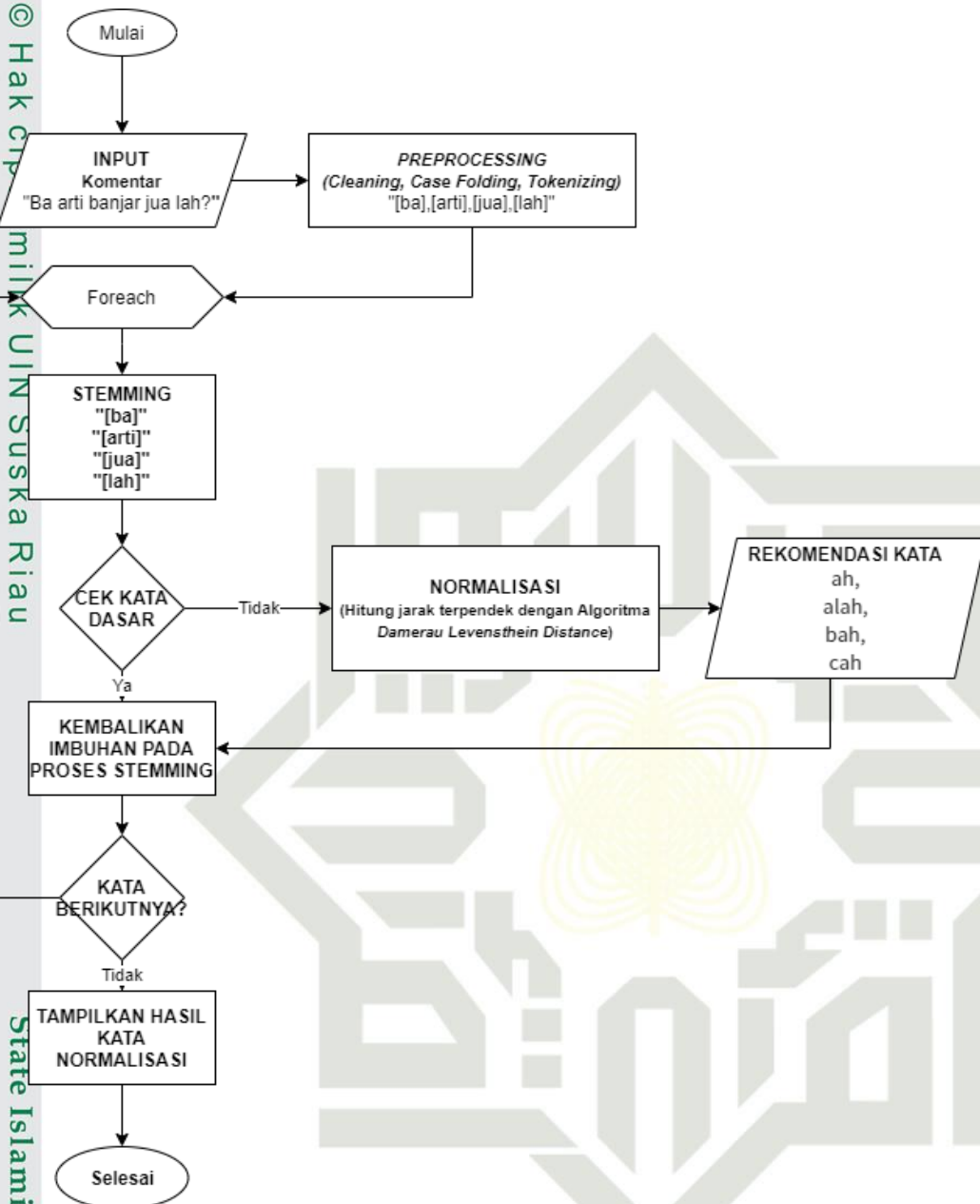
Gambar 3.2 Flowchart Analisa
