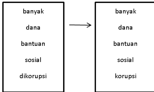
Gambar 3. 7 Contoh Proses Stemming
