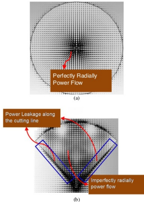
Figs. 2. Power flow within (a) full normal antennas (b) Cut antennas
