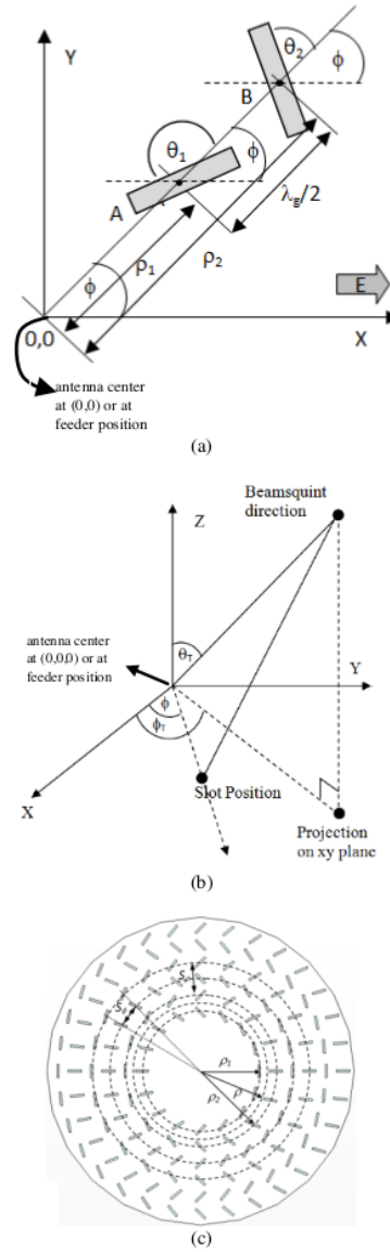
Figs. 5. (a) Slots pairs along with all parameter in x-y plane (b) slots positions and their relations to beam direction in x-y-z (c) distance between slots in radial and azimuth directions [1], [2], [24], [25]
