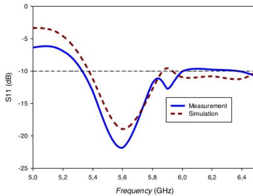
Figure 9. The response of reflection coefficient (dB)
