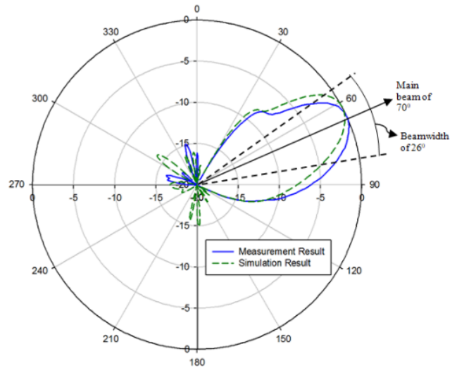
Figure 7. Radiation pattern
