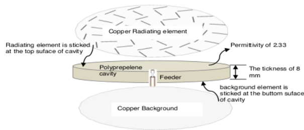
Figure 2. Structures of RLSA antennas
