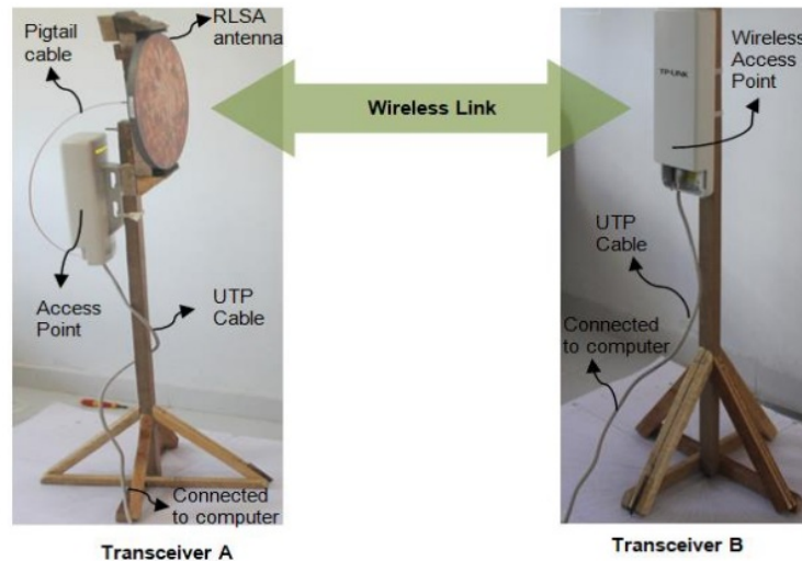
Figure 11. Testbed system
