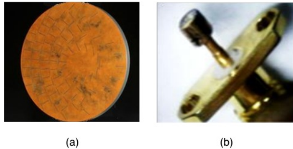
Figure 5. (a) Fabricated antenna (b) Fabricated feeder
