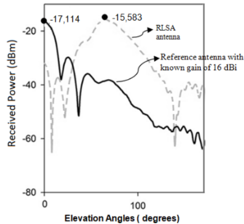
Figure 8. Plot of received power of RLSA and reference antenna
