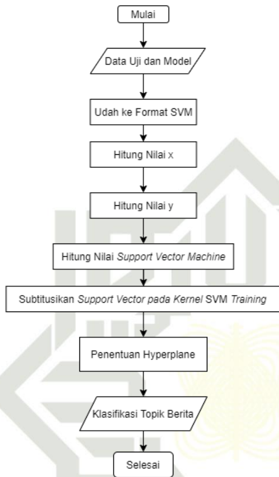
Gambar 3. 3 Proses Metode SVM Data Testing
