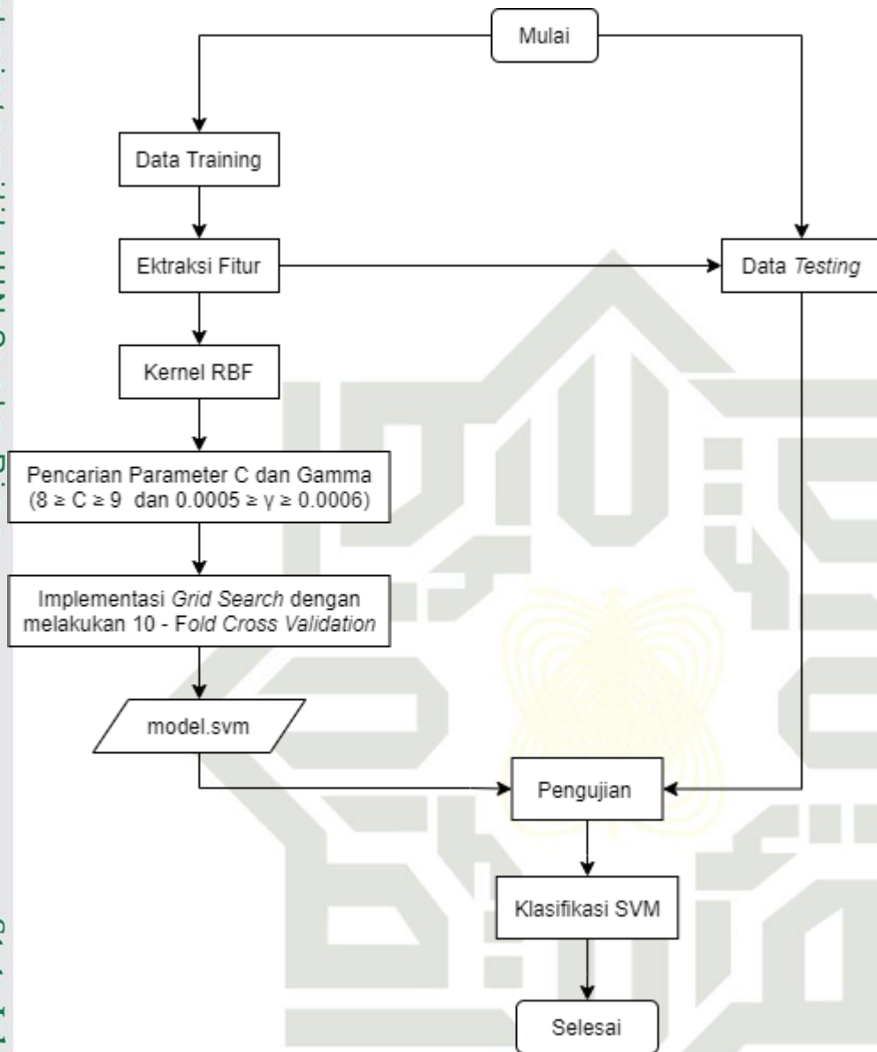
Gambar 4. 9 Analisa Proses SVM
