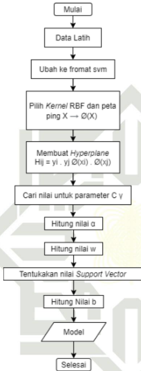
Gambar 3. 2 Proses Metode SVM Data Training
