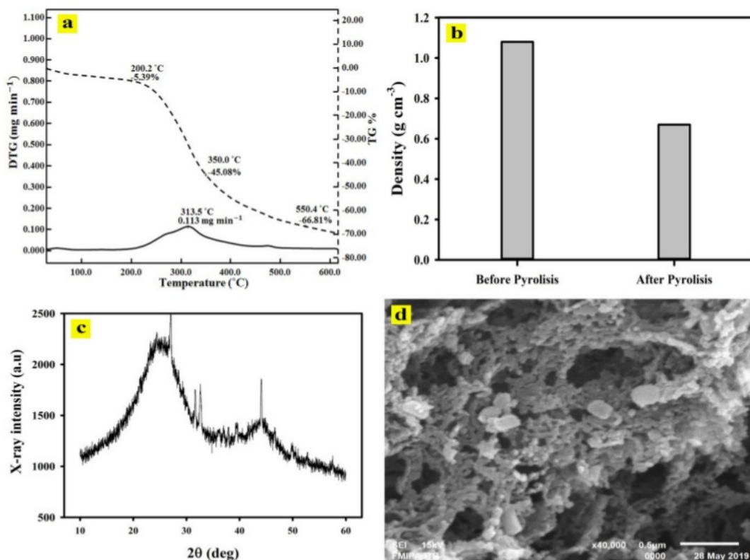
FIGURE 2. (a) TG/DTG curve, (b) density of before and after pyrolysis process, (c) X-ray diffracton pattern for angšana leaves carbon electrode, and (d) SEM with micrograph of 40000x
