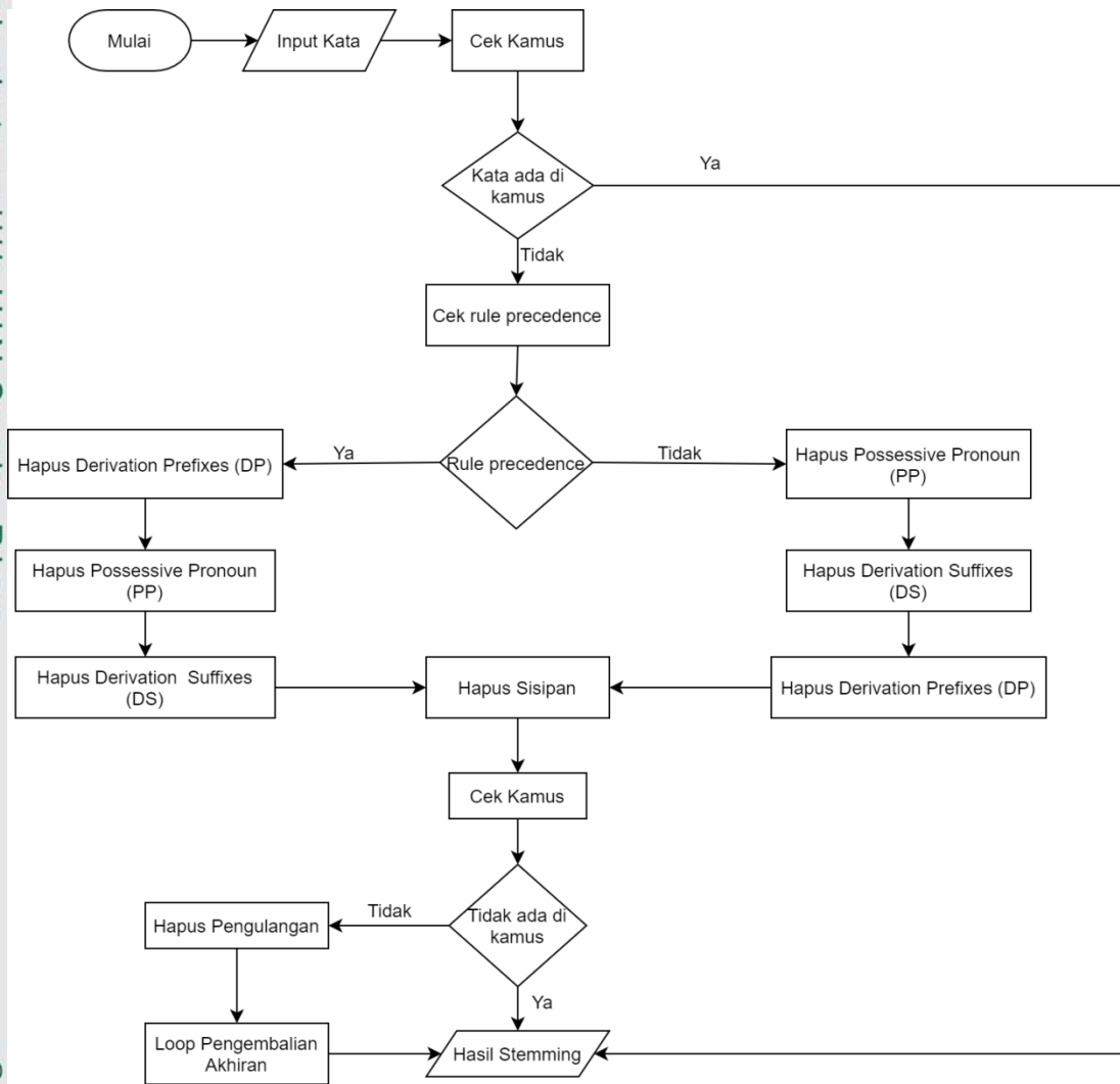
Gambar 3.2 Flowchart Algoritma ECS (Sholihin Andi, 2013)
