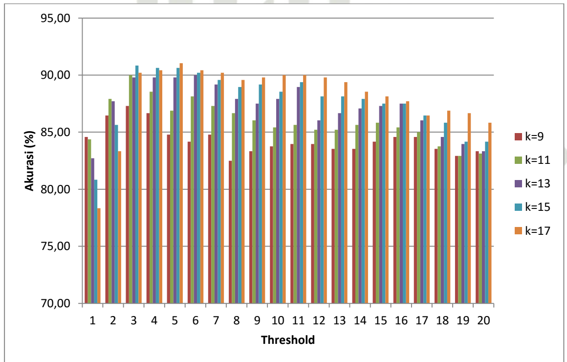
Grafik 5.2 Pengujian Threshold Dataset 80%: 20%
