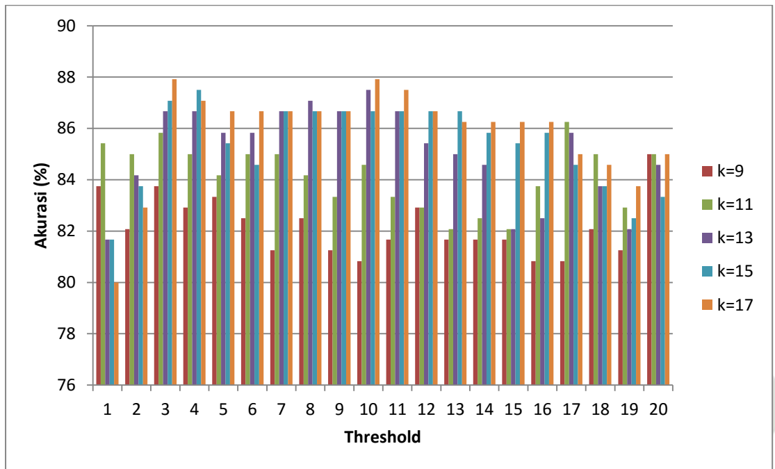
Grafik 5.1 Pengujian Threshold Dataset 90%: 10%
