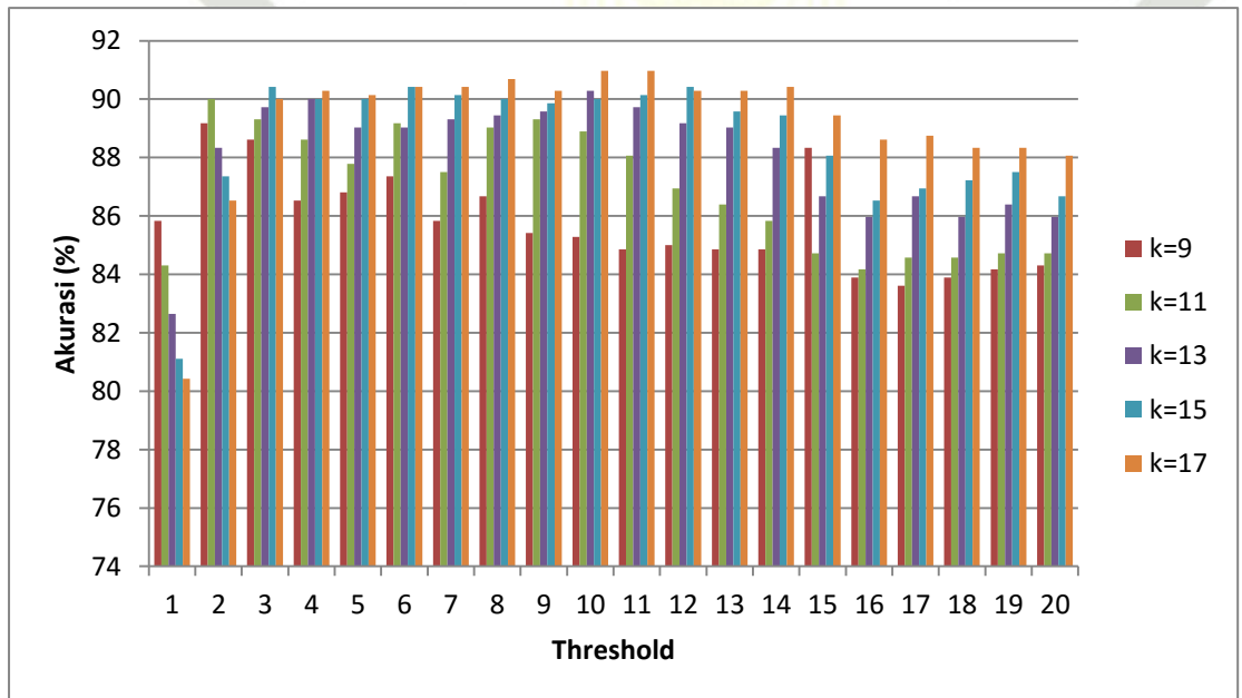
Grafik 5.3 Pengujian Threshold Dataset 70%: 30%
