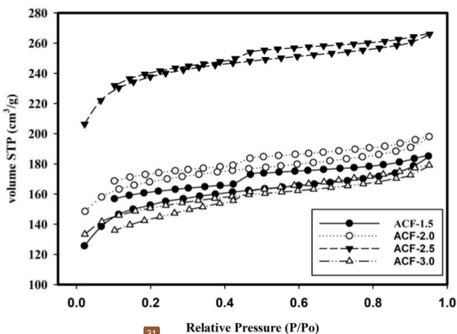
Figure 4. Nitrogen adsorption-desorption isotherms
