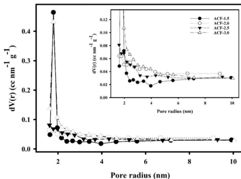
Figure 5. Pore size distribution curves for all samples
