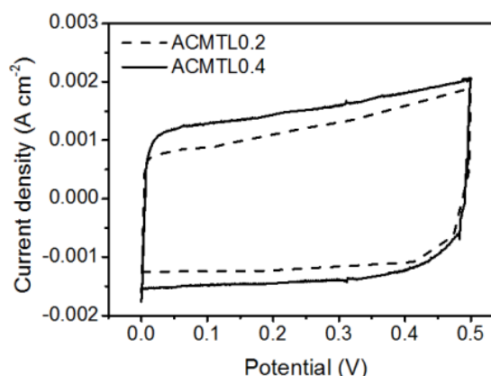
Figure 7: Cyclic Voltammetry curve of the ACMTLx electrodes
