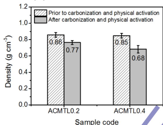
Figure 3: Density of ACMTLx samples
