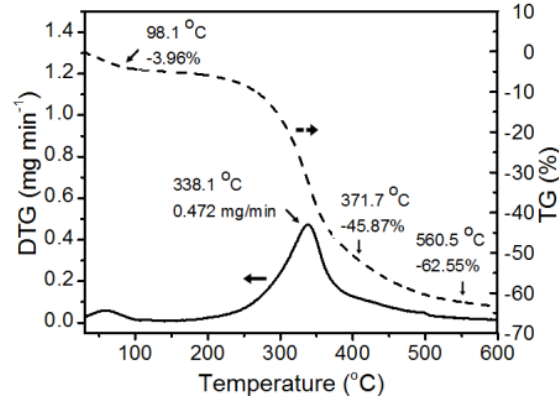
Figure 2: Supramolecular characteristic changes characterized using TGA
