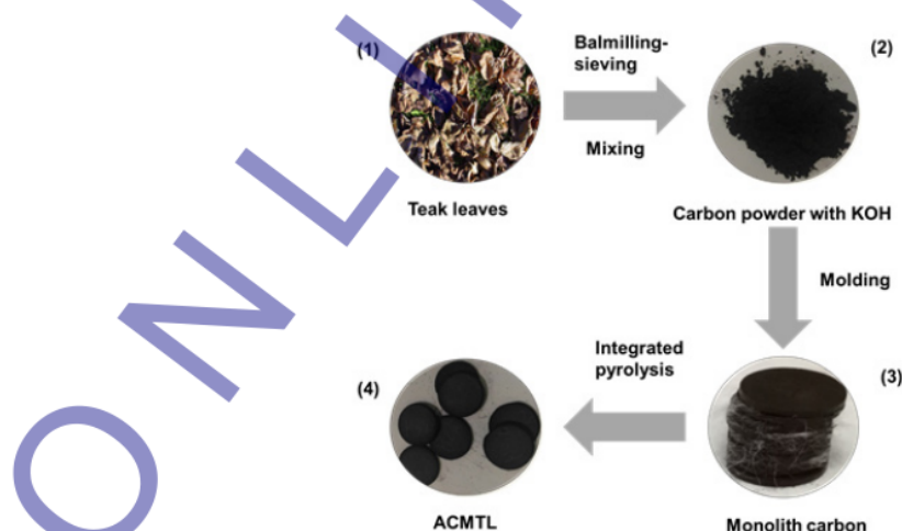
Figure 1: Schematic in ACMTL production
