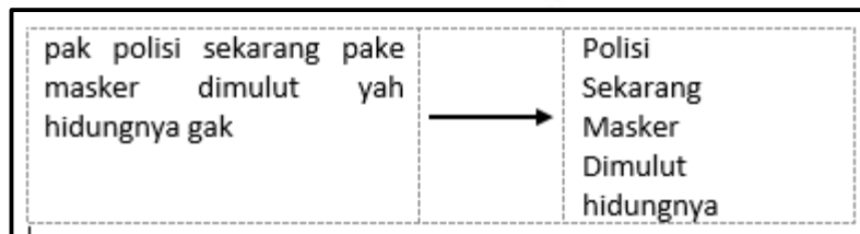
Gambar 2.3 Proses Filtering
