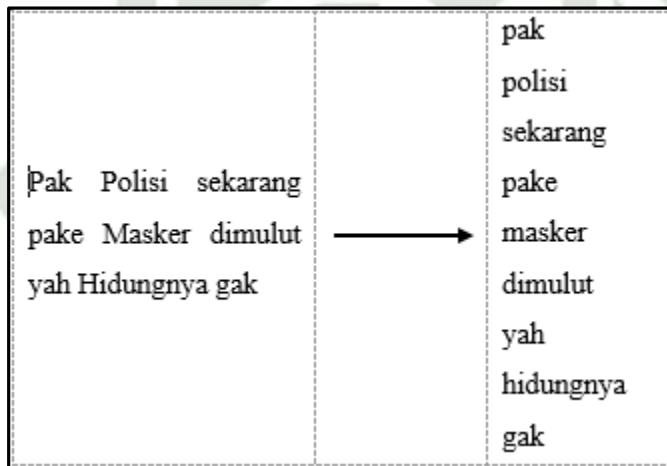
Gambar 2.2 Proses Tokenizing
