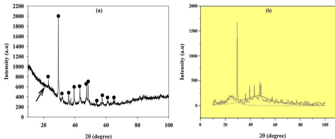
Figure 5. (a) CMWH sample X-ray diffraction pattern, (b) Fittings using microcal origin software
