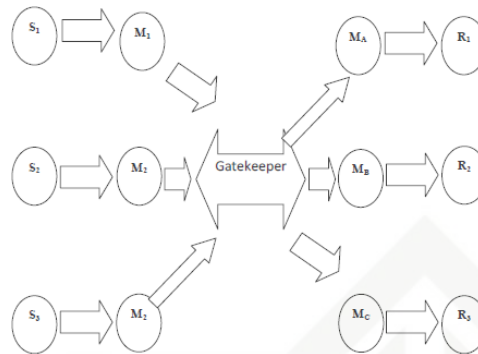
Gambar 2.1 Model Gatekeeper
