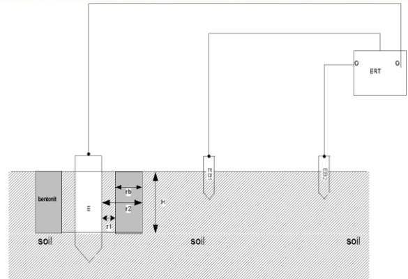
Figure 2. Grounding Resistance Measurement with Salt and Charcoal
