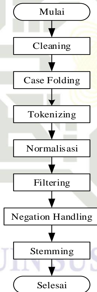
Gambar 4. 2 Flowchart Text Preprocessing
