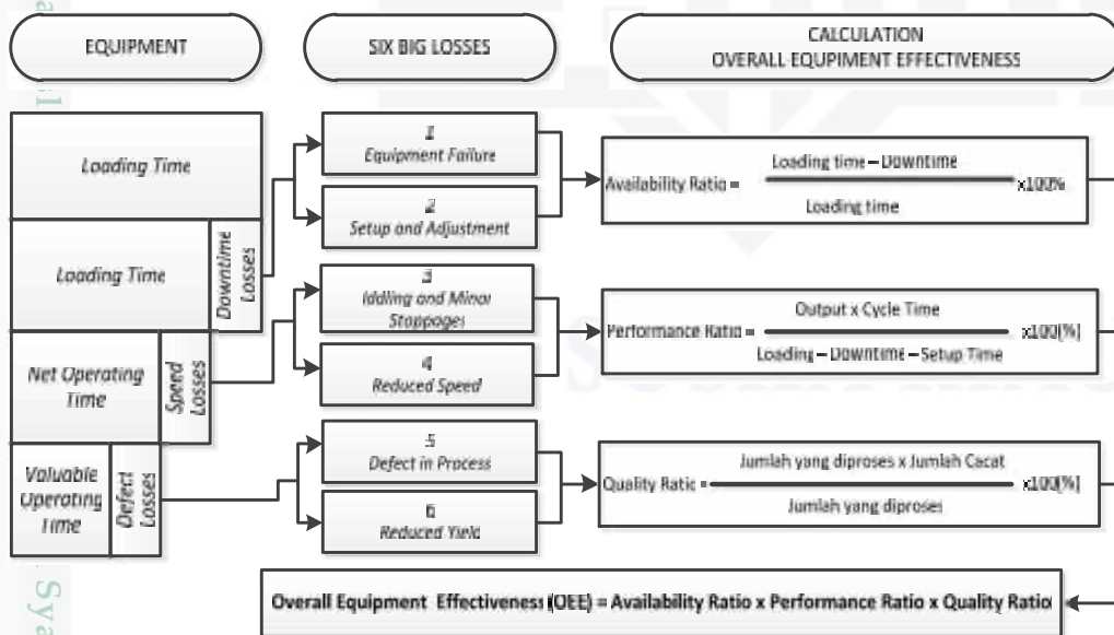
Gambar 2.2 Tahapan Perhitungan OEE
