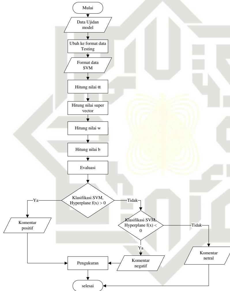
Gambar 4.7 Tahapan SVM Testing
