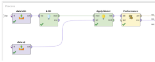
Fig. 4. Rapidminer series for K-NN process
