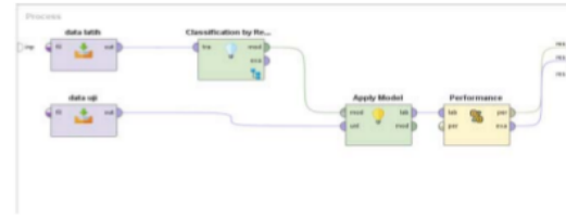
Fig. 5. Rapidminer series for linear regression process
