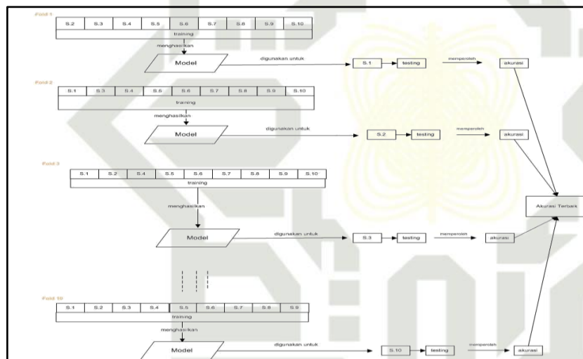
Gambar 4.5 Analisa 10-fold
