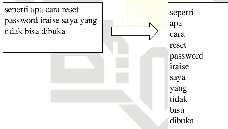
Gambar 4.2 Tahapan Tokenizing
