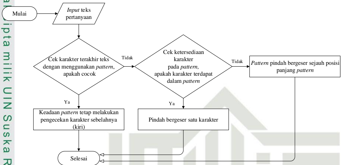
Gambar 4.3 Flowchart Algoritma Boyer Moore
