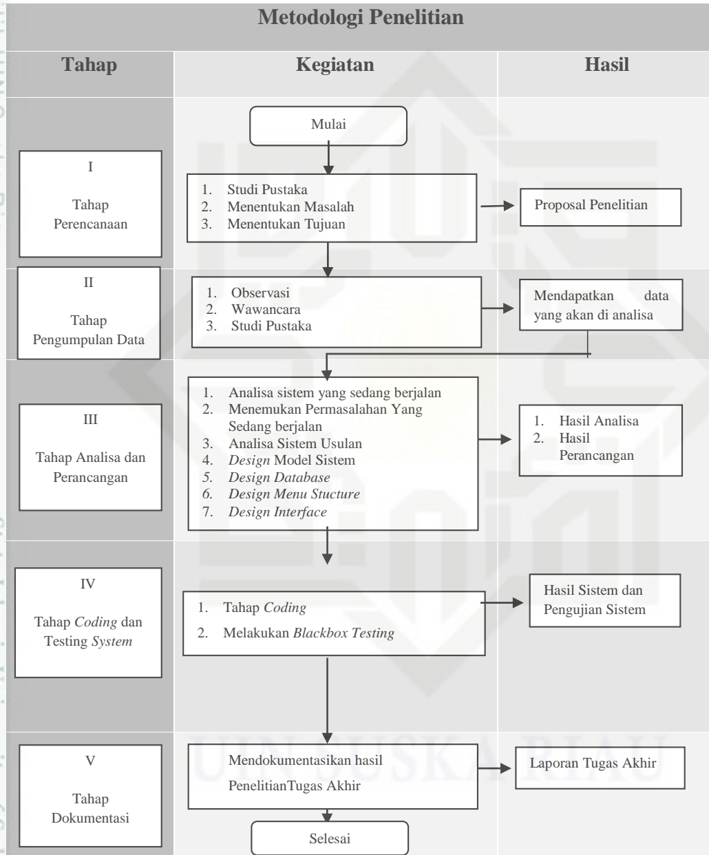
Gambar 3.1. Flowchart Penelitian
