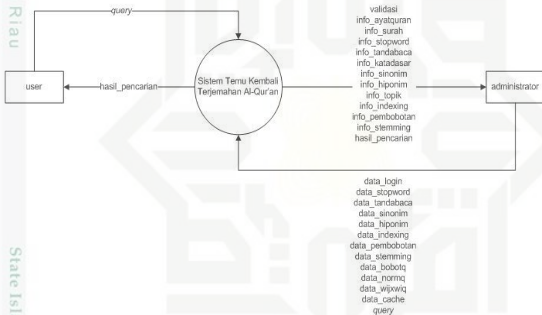
Gambar 4.1 Context Diagram
