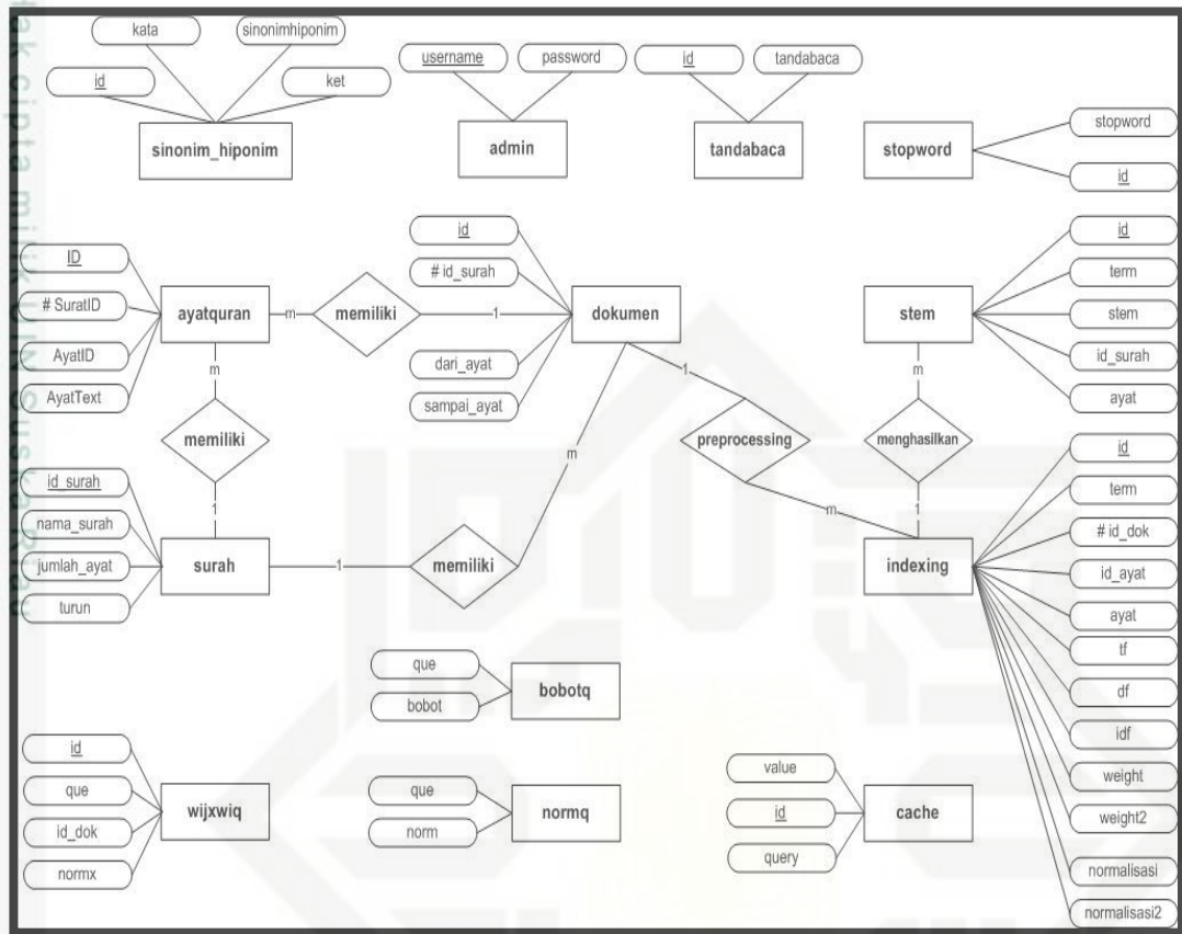
Gambar 4.3 ERD
