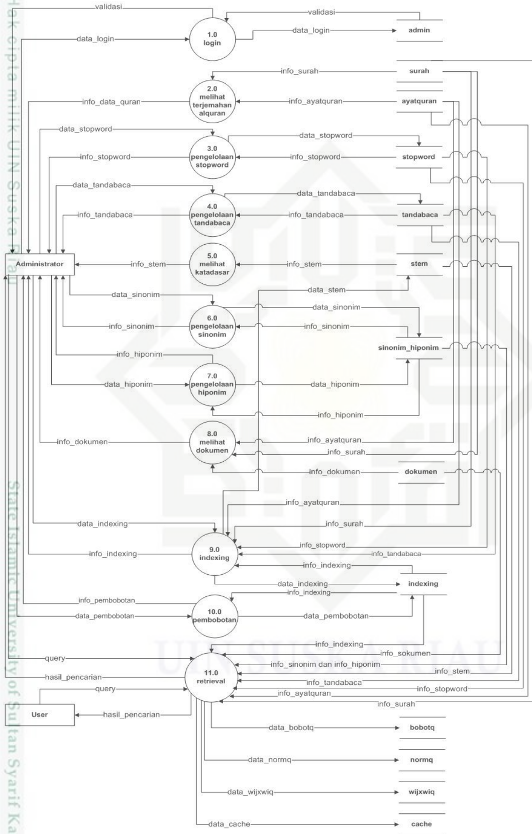
Gambar 4.2 DFD level 1
