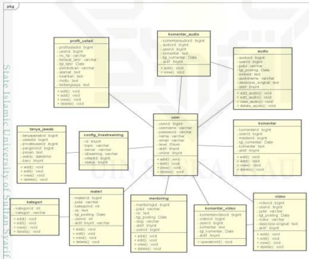
Gambar 4.33 Class Diagram
