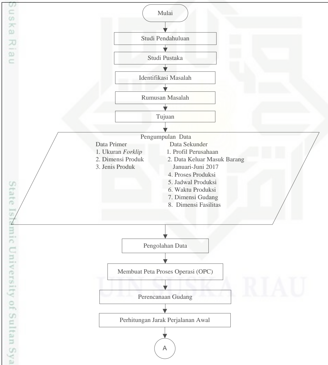
Gambar 3.1 Flowchart Penelitian
